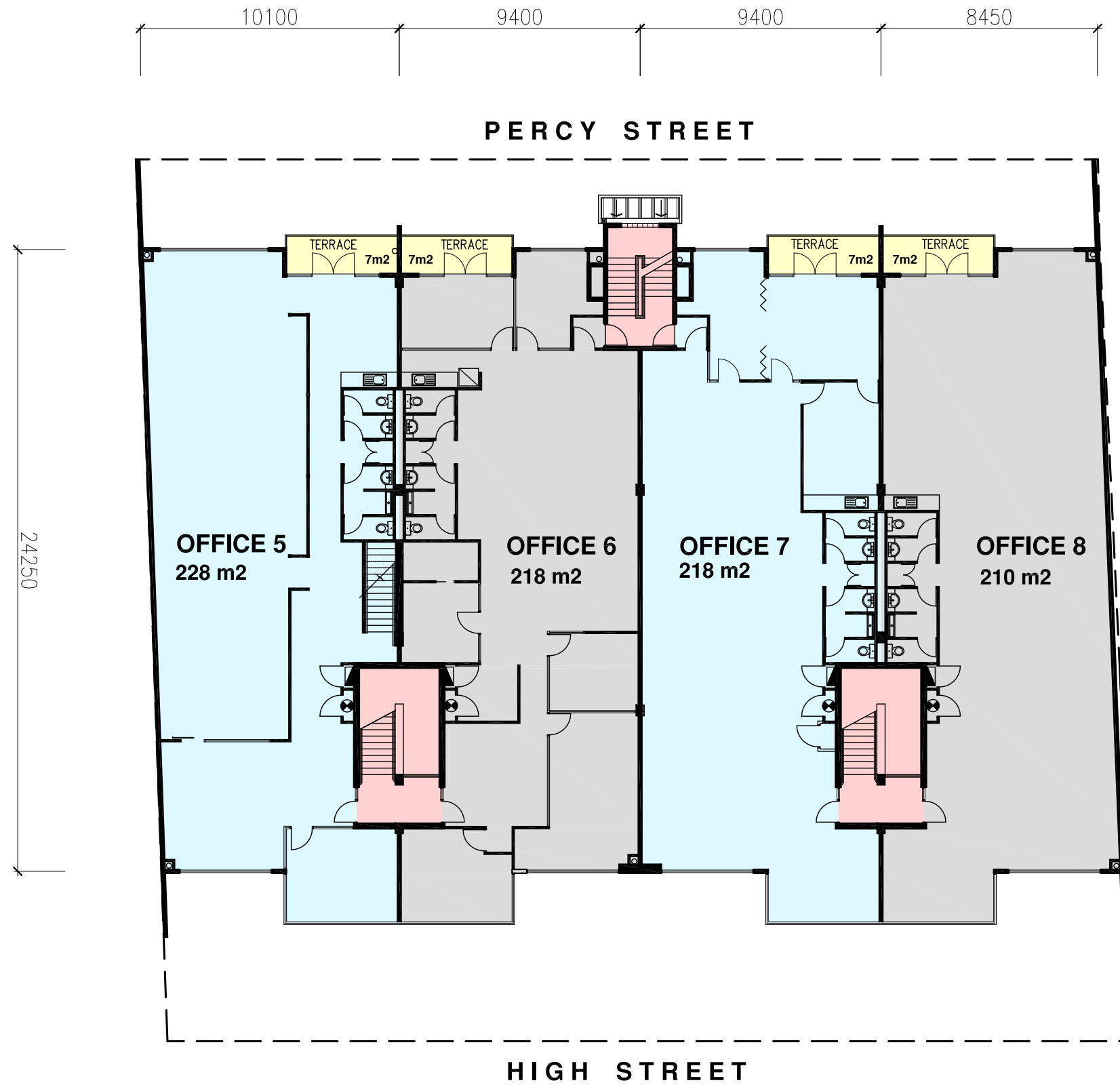
01 FIRST FLOOR PLAN 1:200
